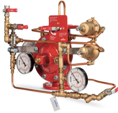
77DE-HRV-PR-MR Manuel Reset
