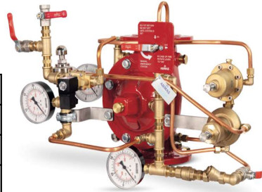
77DE-EL-HRV-PR-MR Manuel Reset
