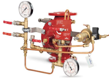
77DE-EL-HRV-MR Manuel Reset
