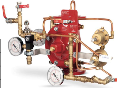
77DE-EL-PORV-PR-MR Manuel Reset
